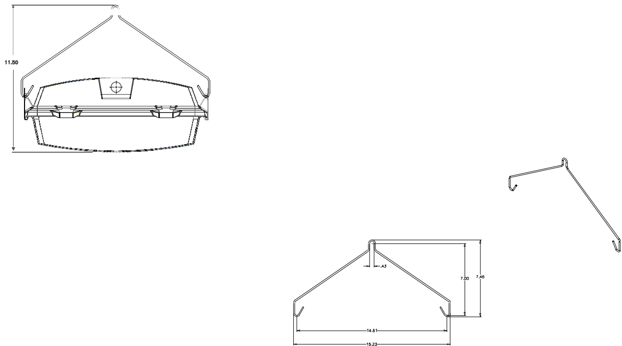
FX7093 (2 each) V Hook for chain or cable mounting (Selection "1" from ORDERING REFERENCES)
