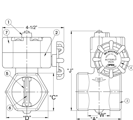
THREADED ENDS BB-SCS02
