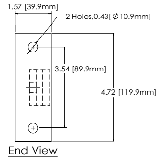
2 - Typical ALOF1GS Wall Bracket Base Not to Scale
