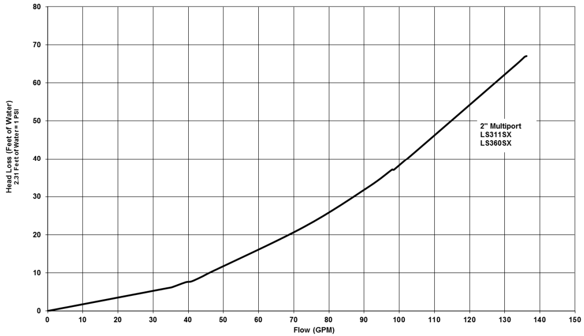
Head Loss Chart
