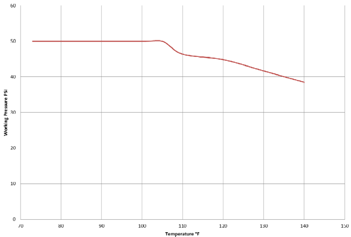
Sand Filter Working Pressure Air or Water Temperature
