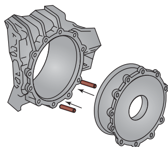
BELL HOUSING POSITIONING ELEMENT
