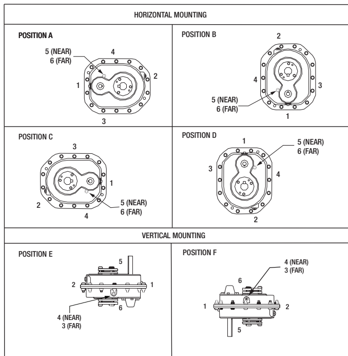
Figure 1 - Mounting Positions
