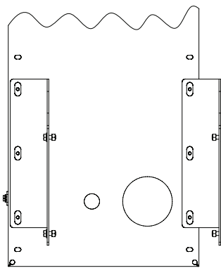
Figure 17 - Mounting Brackets in Position C
