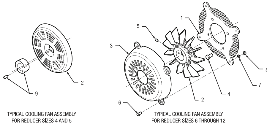
Figure 11 - Parts Identification
