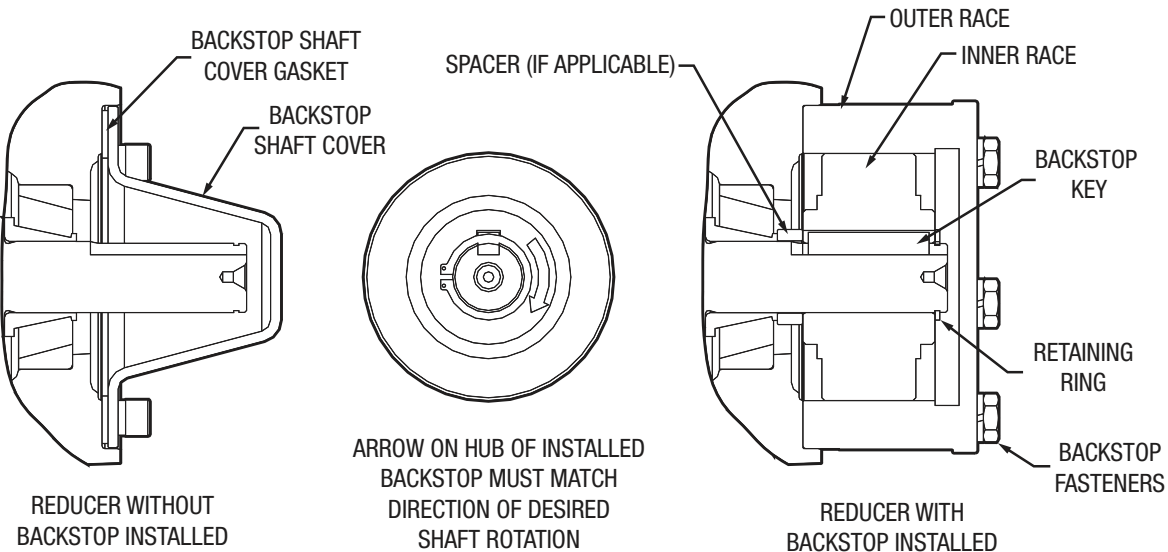
Figure 12 - Backstop Assembly
