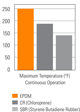
Operating Temperature
