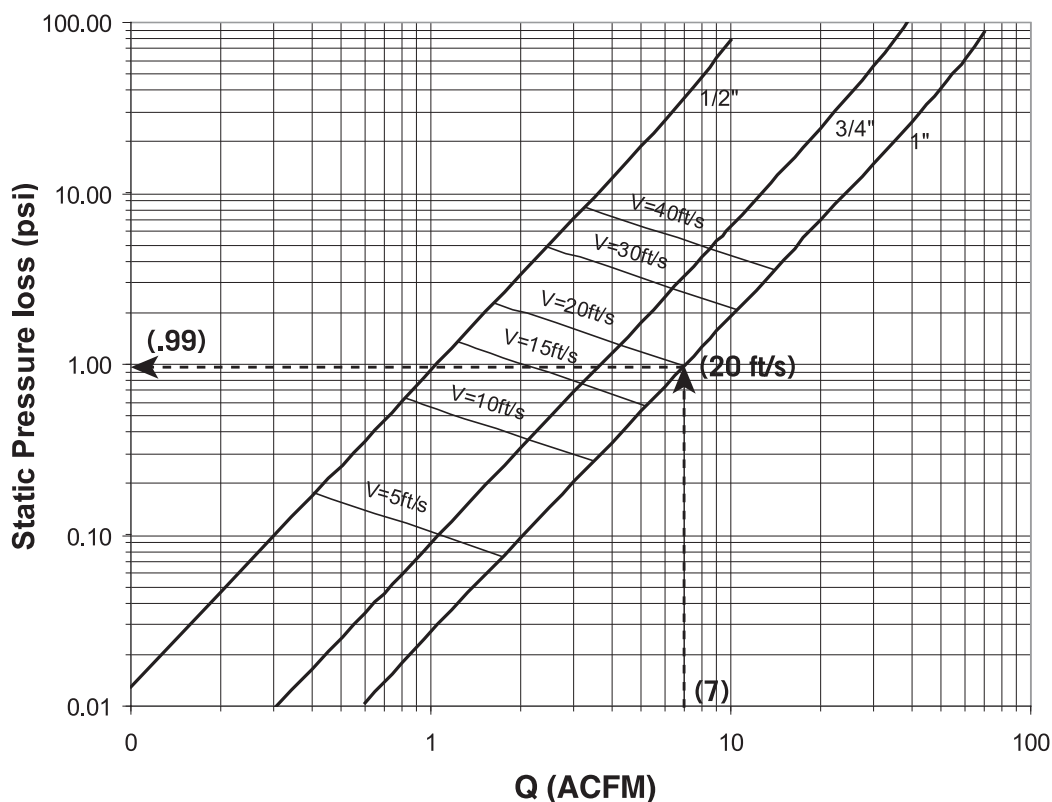
Figure 3 – Pressure Loss per 100 feet of Duratec Pipe Air at 200 psig (214.7 psia), 73°F
