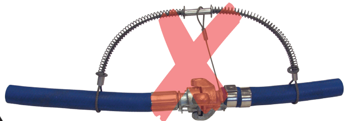
Incorrect Installation
