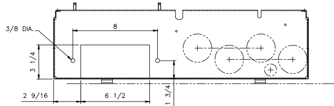
BOTTOM ENDWALL KNOCKOUTS FOR UNITS WITH "T" SUFFIX
