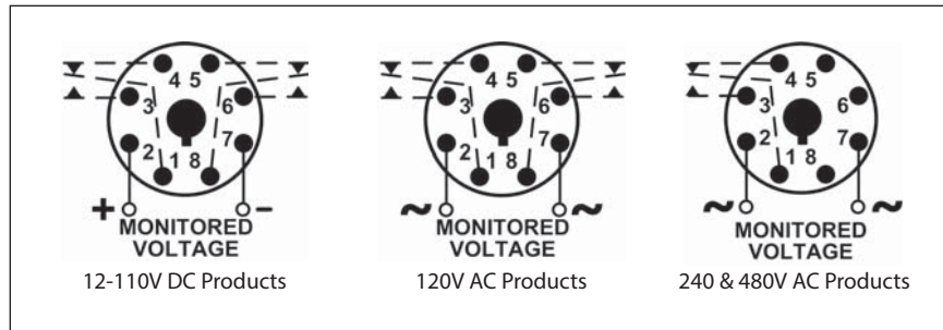
Figure 1. Wiring for 8-Pin Socket
