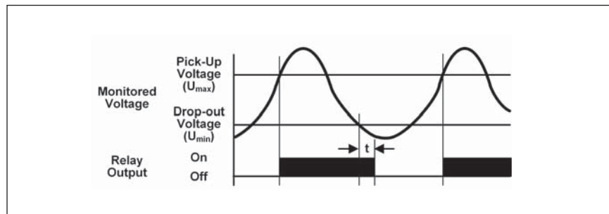
Figure 2. Over/Under Voltage
