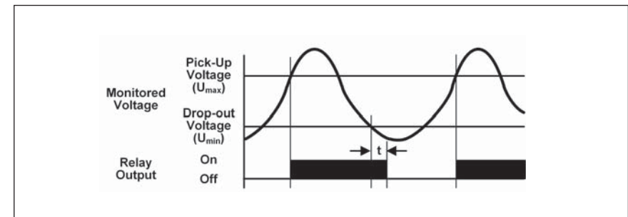
Figure 2. Over/Under Voltage
