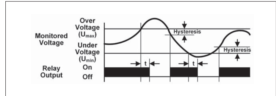
Figure 3. Voltage Band
