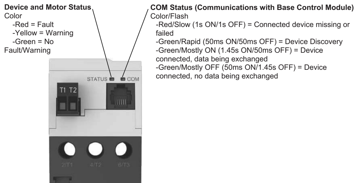
Figure 56. Measurement Module LED Overview
