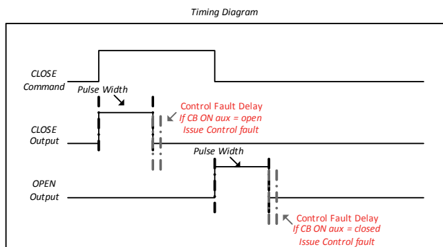
Figure 98. Timing Diagram for MCCB Feeder Operation Mode
