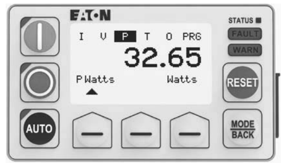
Figure 99. C445UM: Monitoring User Interface
