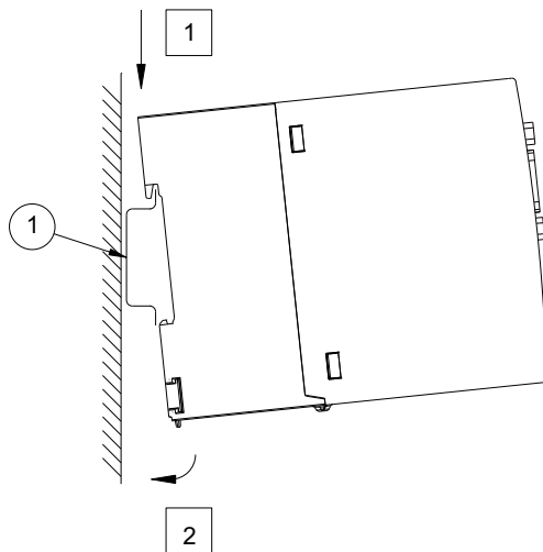
Figure 20. DIN-Rail Mounting Instructions
