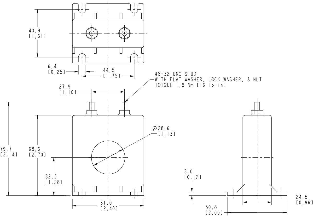
Figure 30. C445XG-CT2—28 mm Diameter Zero Sequencing Ground Fault CT
