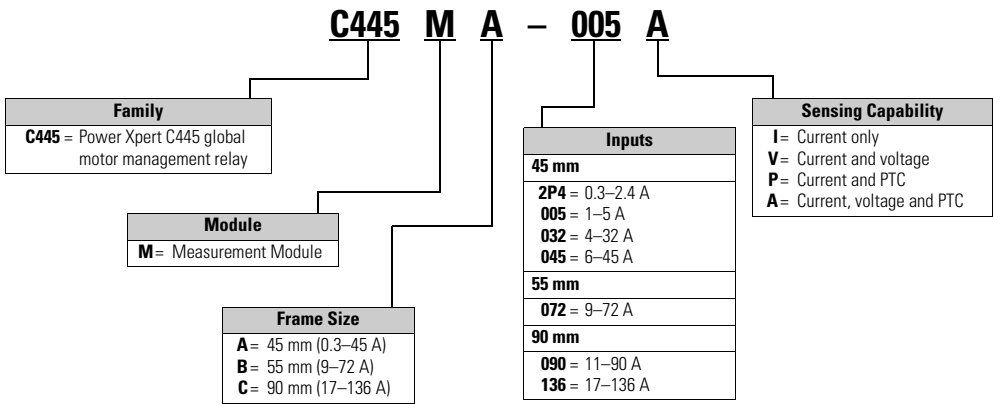
Figure 3. Measurement Module Catalog Numbering
