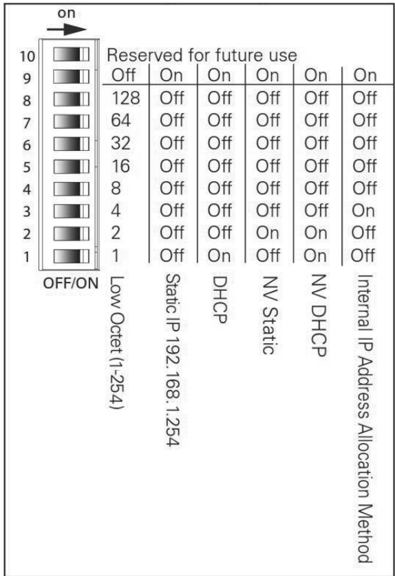
Figure 132. Base Control Module DIP Switches with Ethernet Card
