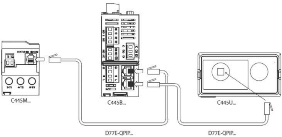
Figure 57. C445 System Connection
