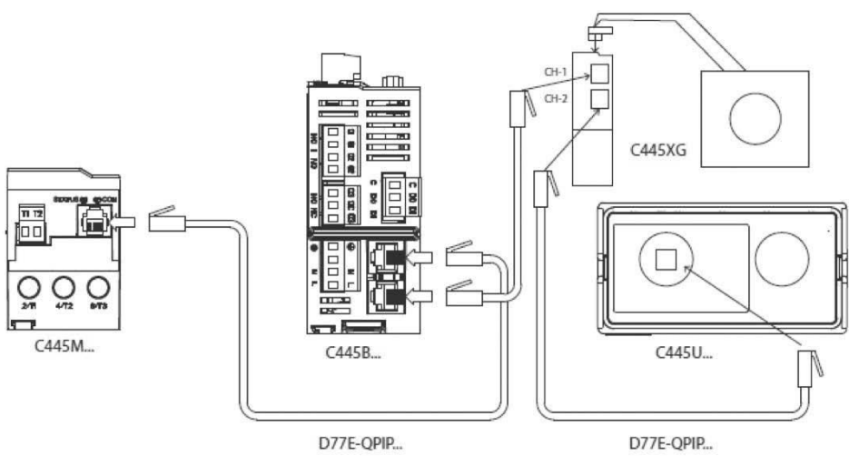
Figure 58. C445 System Connection with Ground Fault Included
