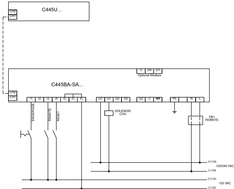
Figure 97. 120 Vac Inputs and 120/230 Vac Outputs/C445 Power
