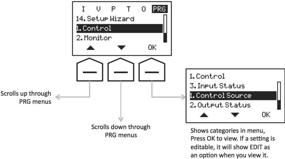
Figure 123. C445UM Program Menu
