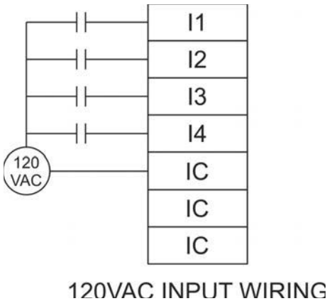
Figure 45. 120 Vac Input Terminal Diagram
