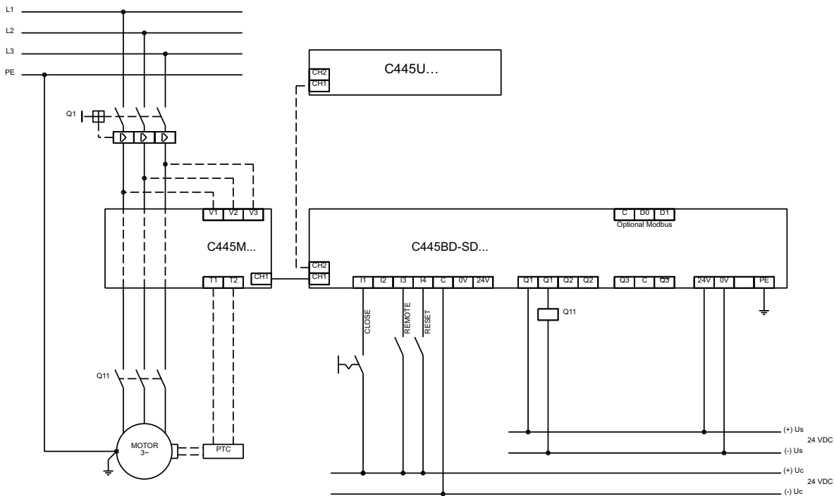
Figure 105. Isolated 24 Vdc Inputs/24 Vdc Outputs/24 Vdc Power
