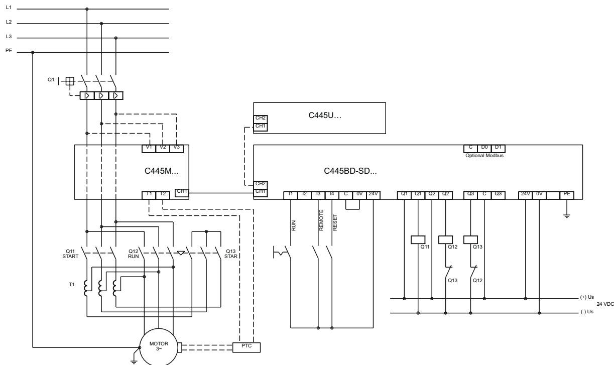
Figure 91. Non-isolated 24 Vdc Inputs/24 Vdc Outputs/24 Vdc C445 Power
