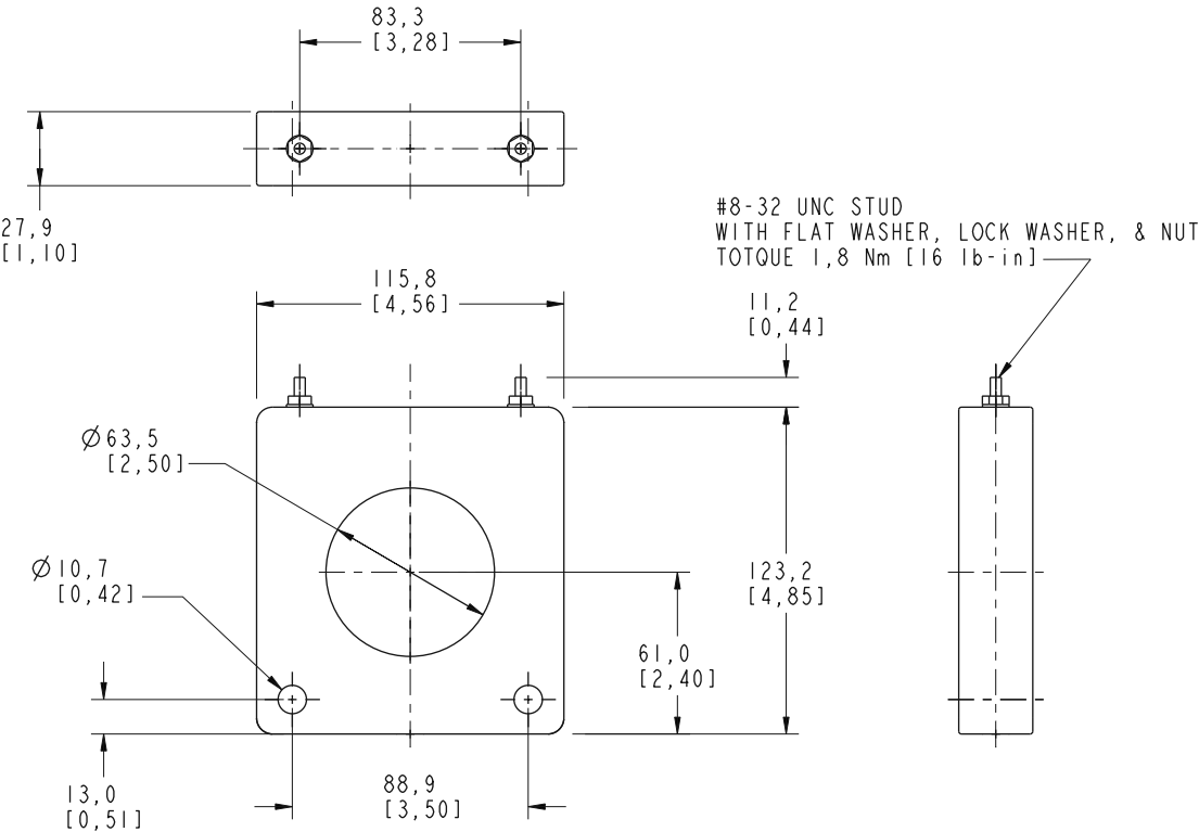
Figure 32. C445XG-CT4—63 mm Diameter Zero Sequencing Ground Fault CT
