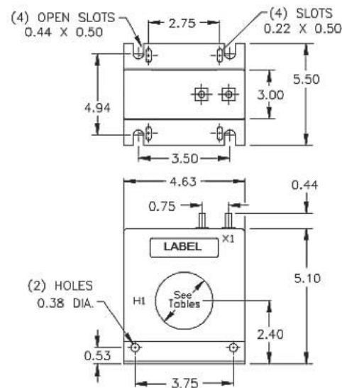
XCT800-5 (inches)
