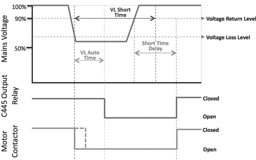
Figure 114. Example #3: Short-Time—Mains Voltage Returns Before Short Time Expires
