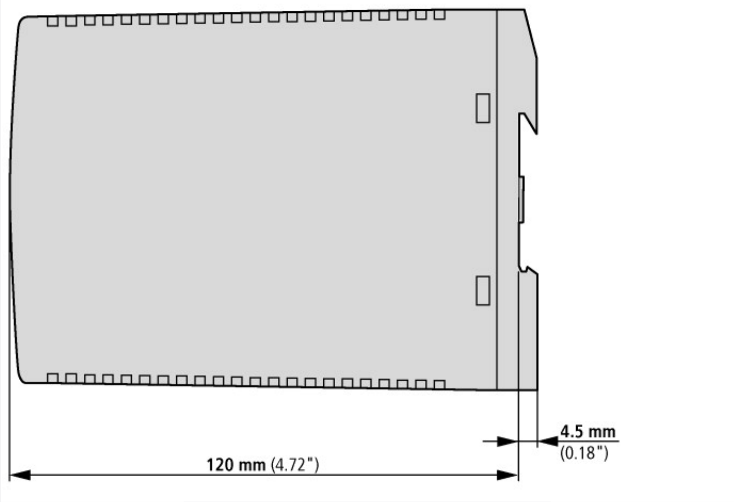
SmartWire-DT Gateways
