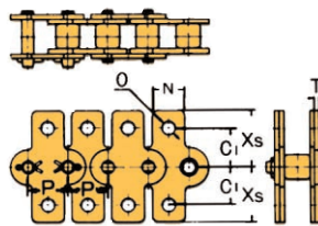
SKK-1 Attachment
