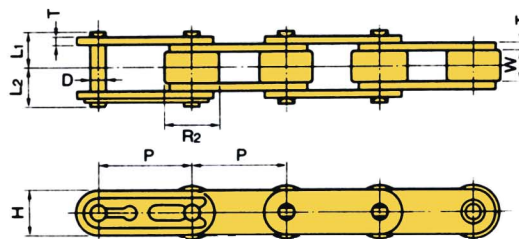
Oversize "R" Roller Type
