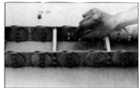
Insert the pin and lock in place with the retaining ring.
