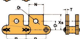
SK-1 Attachment
