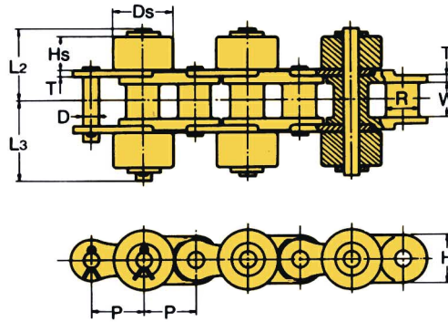
Type II (Crosswise Installation)
