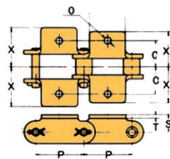
K-1 Attachment
