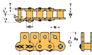
SK-1 Attachment
