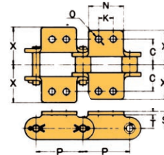
K-2 Attachment
