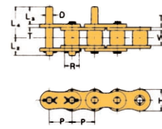
D-1 Attachment
