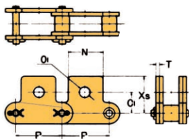
SK-1 Attachment
