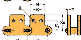
SK-2 Attachment
