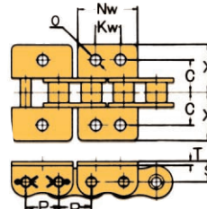
WK-1, WK-2 Attachment
