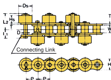
Type I (Staggered Installation)
