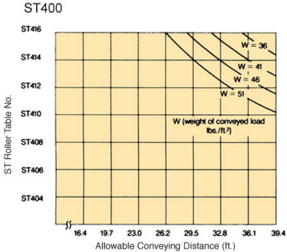
ST Roller Table Conveyor Capability Graph
