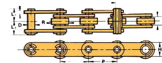
Double Pitch Type – Oversize "R" roller type
