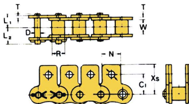
SK-1 Attachment
