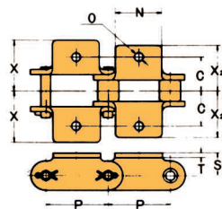
K-1 Attachment
