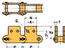
SK-2 Attachment
