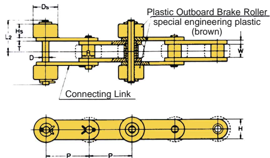
Type II (Crosswise Installation)
