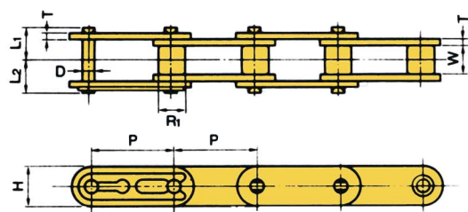
Standard "S" Roller Type
