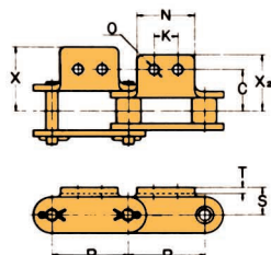
A-2 Attachment
