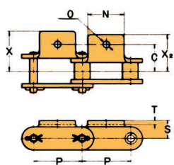
A-1 Attachment
