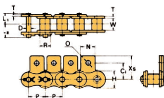
SA-1 Attachment
