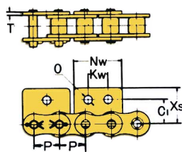
WSA-1, WSA-2 Attachment
