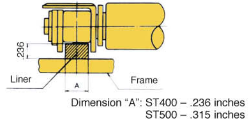
Guide for ST Roller Table
