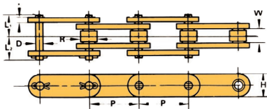
STANDARD "S" ROLLER TYPE
