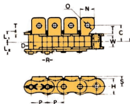
A-1 Attachment
