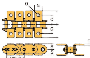
KK-1 Attachment
