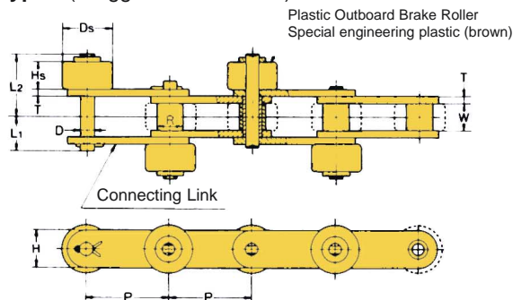
Type I (Staggered Installation)
