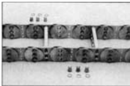
Align the holes on both sides of the chain.
