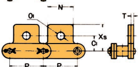
SA-1 Attachment
