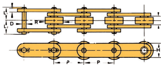
OVERSIZE "R" ROLLER TYPE
