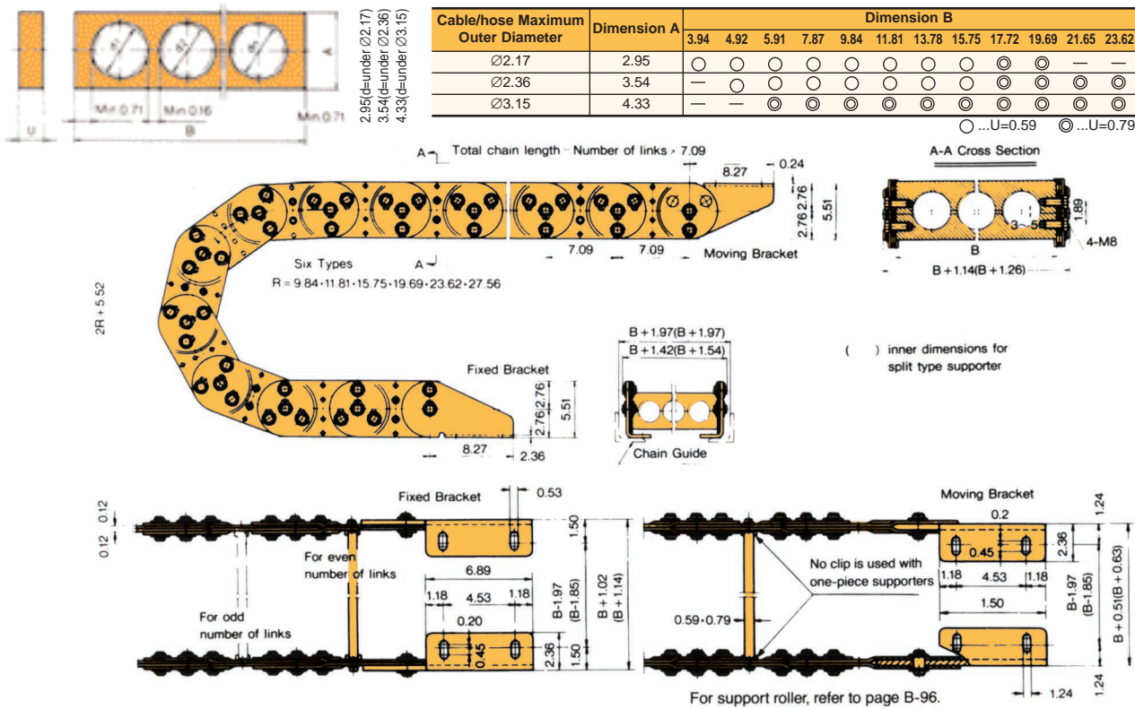
DIMENSIONS FOR STANDARD SUPPORTER
