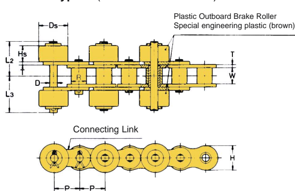
Type II (Crosswise Installation)
