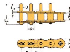
D-3 Attachment
