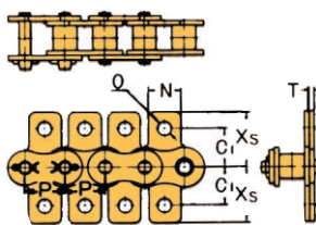
SAA-1 Attachment
