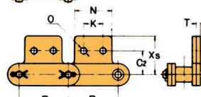
SA-2 Attachment
