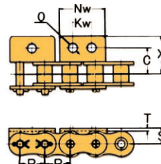
WA-1, WA-2 Attachment
