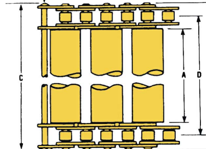
Live Tubular Roller Conveyor Chain Section
