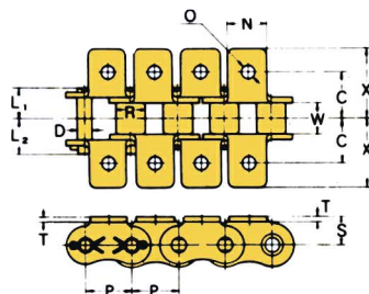
K-1 Attachment
