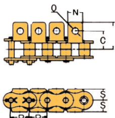
AA-1 Attachment
