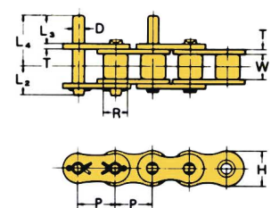
D-1 Attachment
