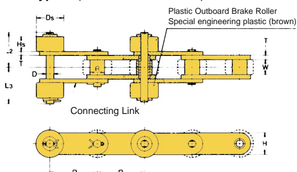
Type II (Crosswise Installation)
