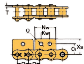
WSA-1, WSA-2 Attachment
