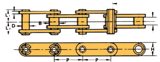
Double Pitch Type – Standard "S" roller type
