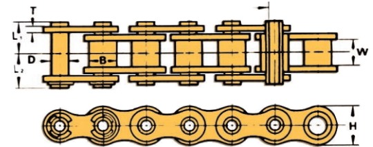
RS Type (Single pitch type)
