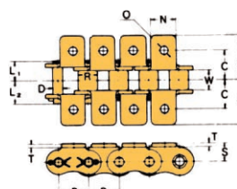
K-1 Attachment
