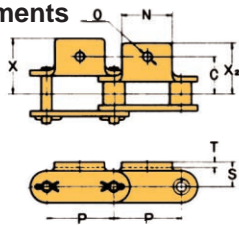
A-1 Attachment
