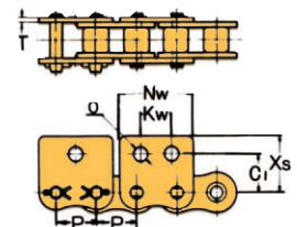
WSK-1, WSK-2 Attachment
