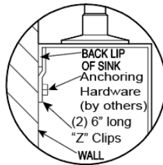
"Z" CLIP DETAIL
