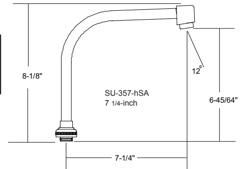
A8 - Suffix 7 1/4-inch High-Rise Swivel Spout
