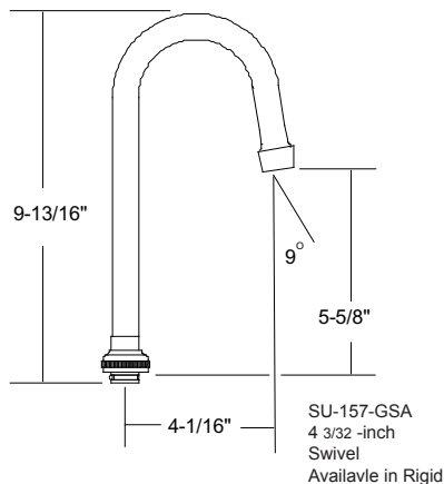
GSA - Suffix 4 3/32 Swivel Gooseneck Spout GRA - Suffix 4 3/32 Rigid Gooseneck Spout
