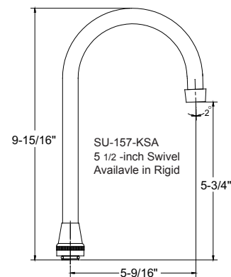
KSA - Suffix 5 1/2 Swivel Gooseneck Spout KRA - Suffix 5 1/2 Rigid Gooseneck Spout
