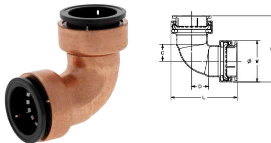
P607 90° Elbow - Push x Push
