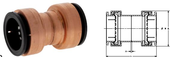
P600 Coupling - Push x Push
