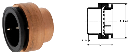
P617 Cap - Push
