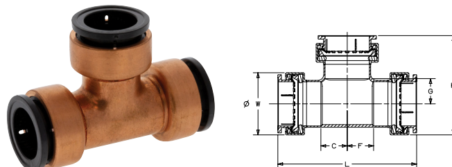
P611 Tee - Push x Push x Push
