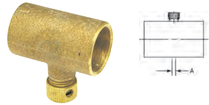
701-D ⚠ Drain Coupling C x C – Cast
