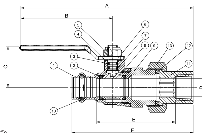
PCFU-FP-600A-LF Press x FIP Union 1/2" - 1"
