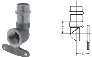
PC707-3-5-A Hi-Ear Elbow P x F – Cast *Lead Free
