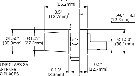
Typical for Bus Bar Termination (Side View)
