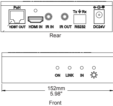
Transmitter and Receiver dimensions (Transmitter shown)
