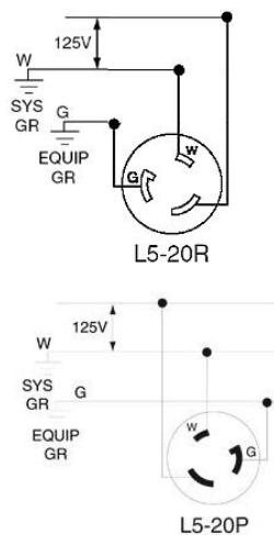
Wiring Diagram
