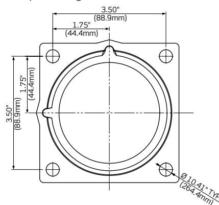
Panel Receptacle Flange
