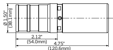
Female Contact
