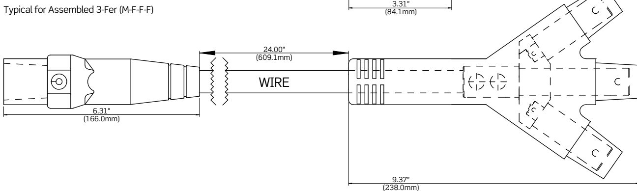
Typical for Assembled 3-Fer (M-F-F-F)
