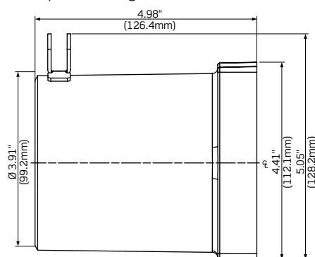
Panel Receptacle Housing
