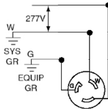
Wiring Diagram
