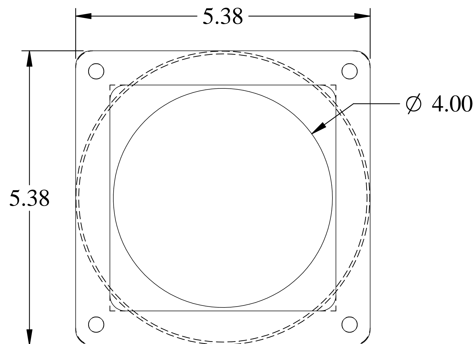
END VIEW
