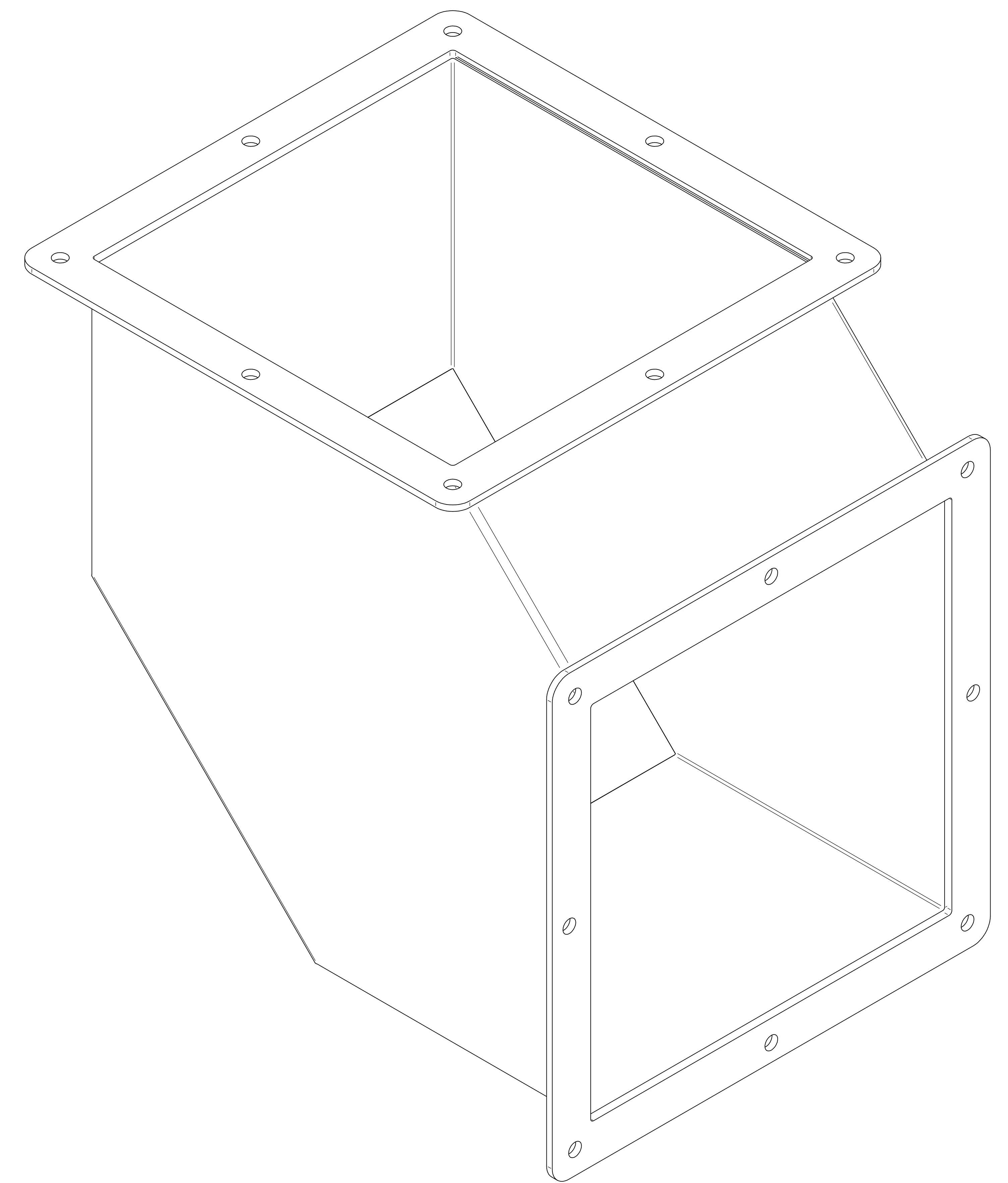
ISOMETRIC VIEW
