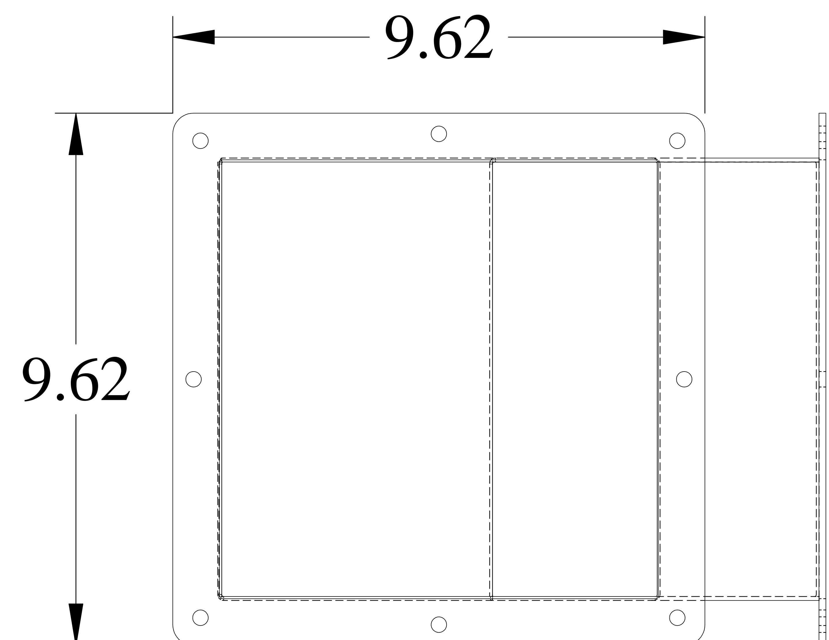
END VIEW
