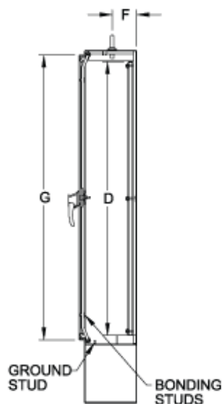
Section X-X
