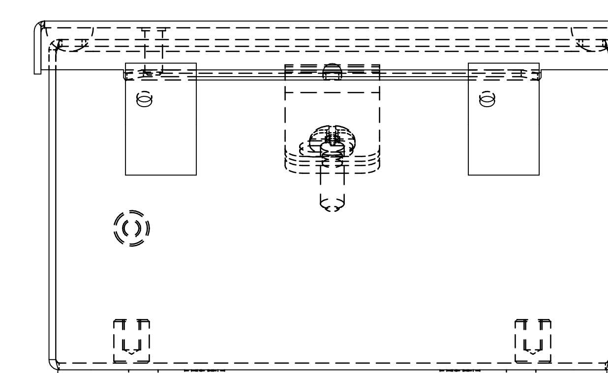
BOTTOM VIEW
