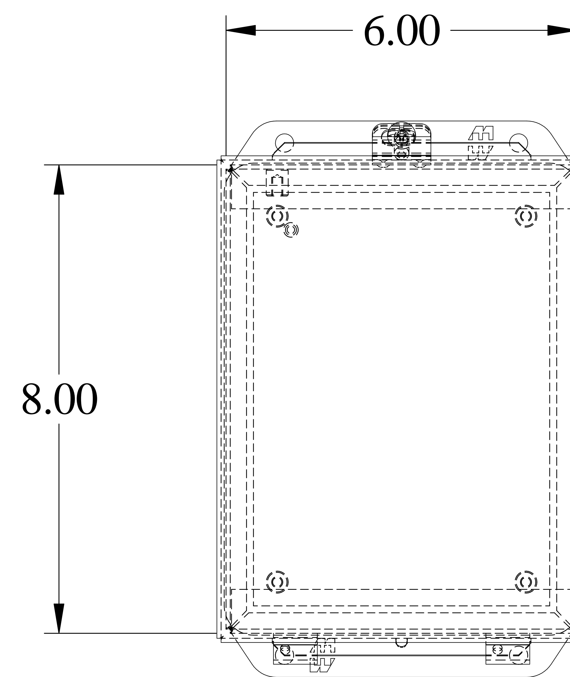
FRONT VIEW
