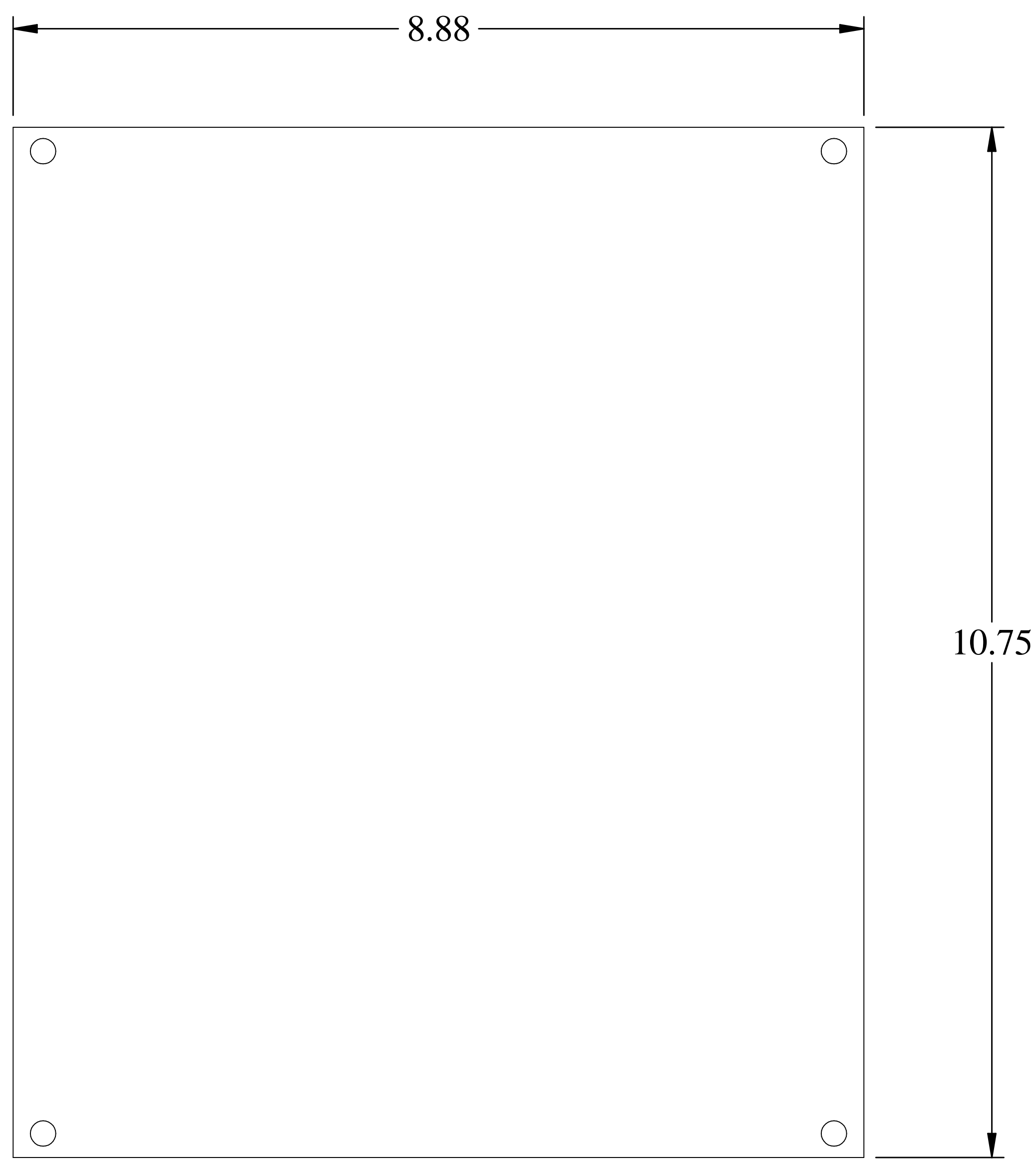
INNER PANEL
