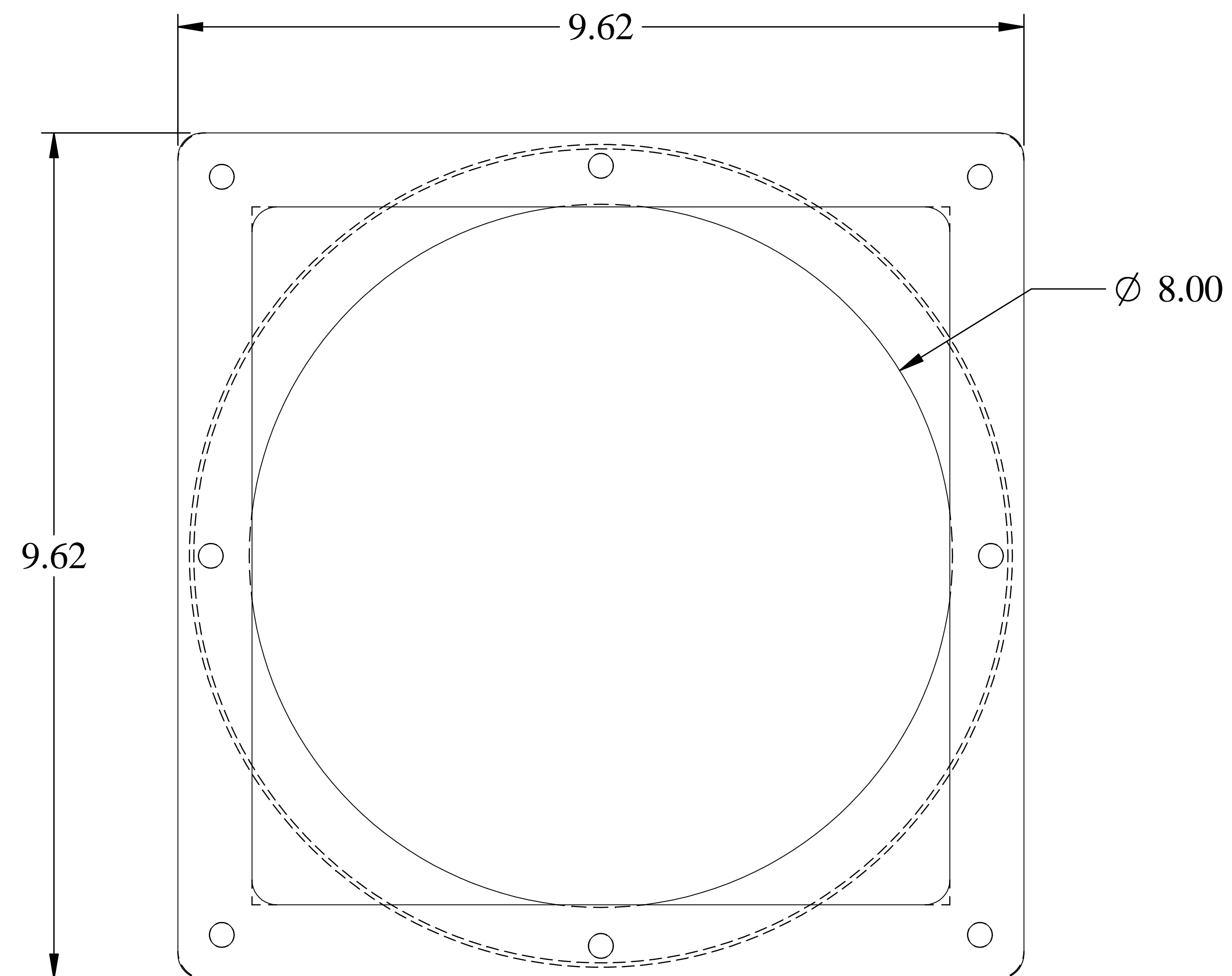
END VIEW
