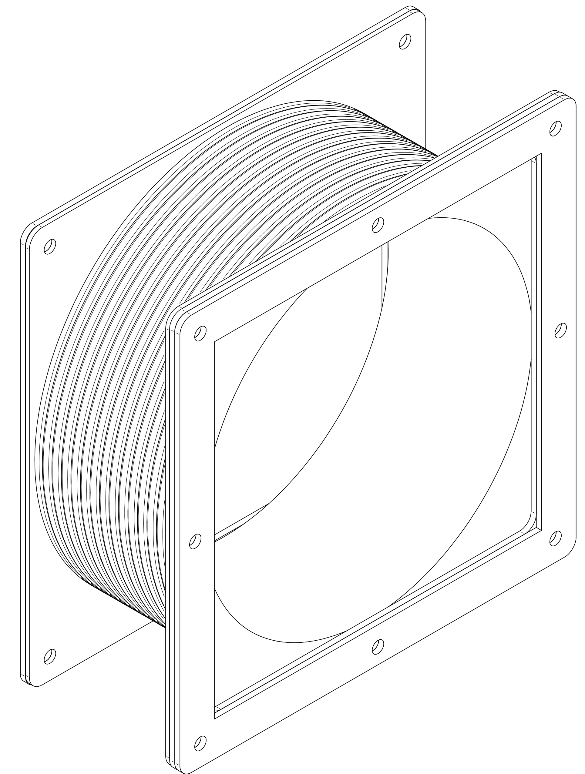
ISOMETRIC VIEW
