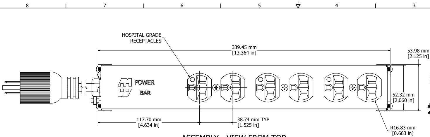
ASSEMBLY - VIEW FROM TOP
