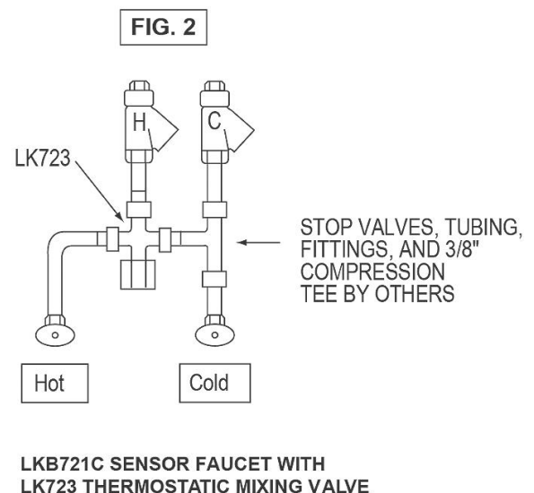
DOUBLE STATION ROUGH-IN
