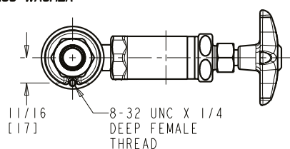
TOP VIEW LESS WASHER
