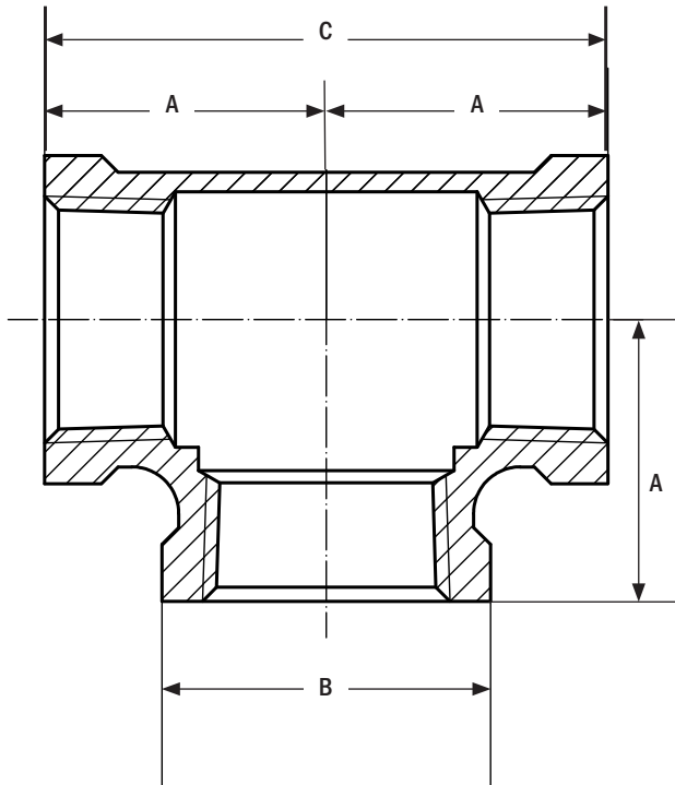
Stainless Steel Tee - 2230SS
