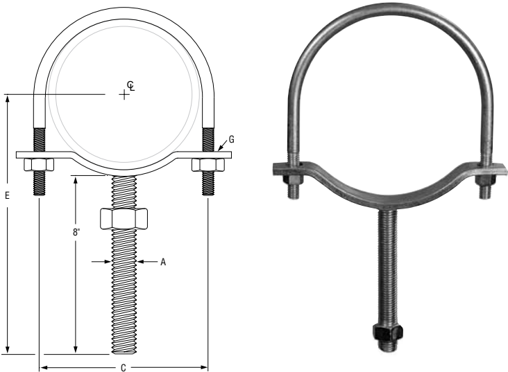
Adjustable Pipe Saddle with U-Bolt
