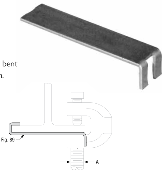
FIG. 89: RETAINING CLIP: WEIGHT (LBS) • DIMENSIONS (IN)
