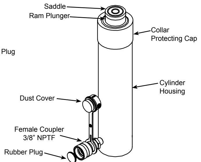
Figure 2 - Typical Cylinder Components
