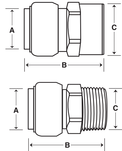
SharkBite® Water Heater Kit Dimensions
