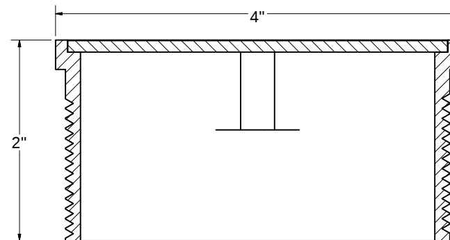
SECTION A-A SCALE 1.5
