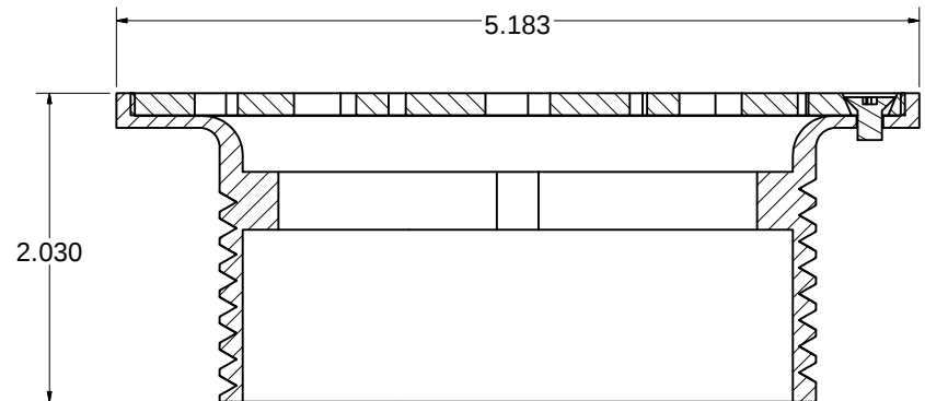
SECTION A-A SCALE 1.5
