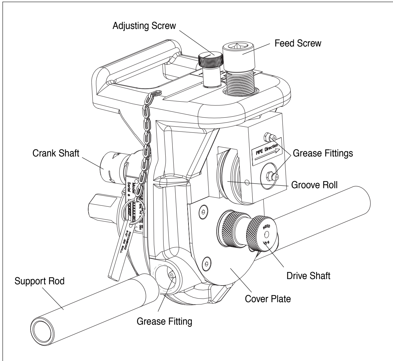
Figure 1 - RGCOMBO2 Roll Groover
