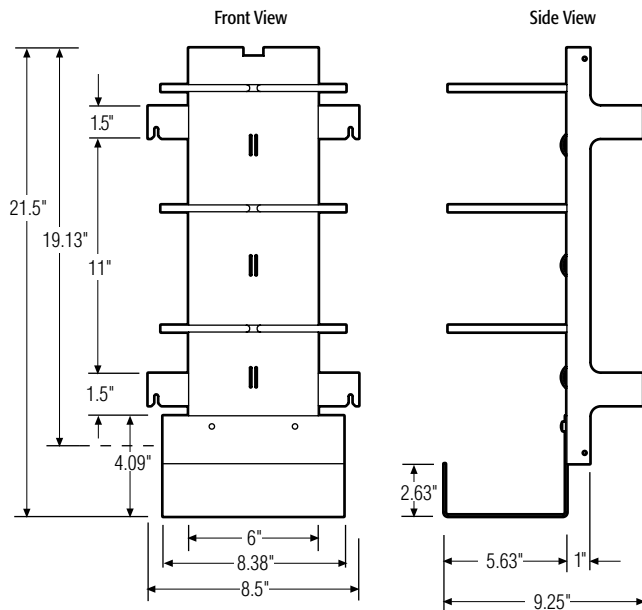
300 Pair Vertical Cord Manager for Basic Units
