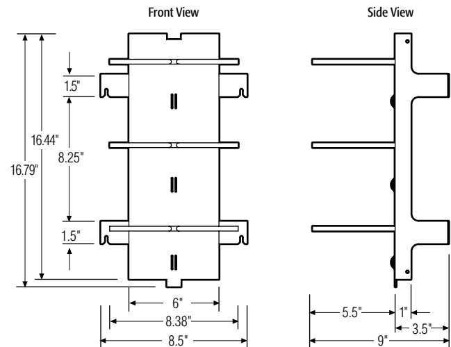
300 Pair Vertical Cord Manager for Extension Units
