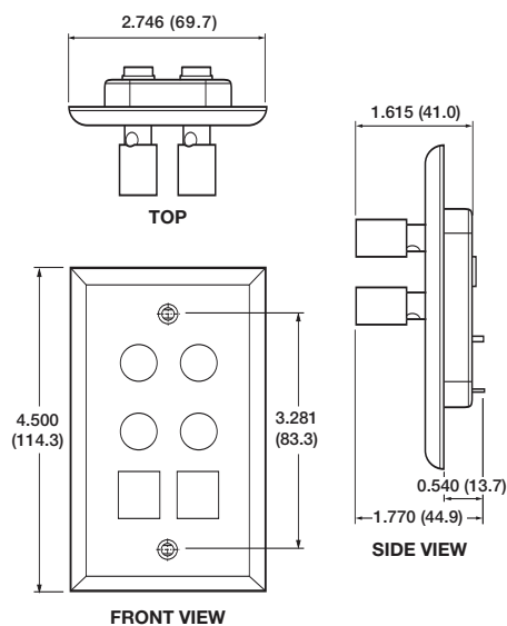
Multi-Room Wallplate (Cat. No. AEMRK)
