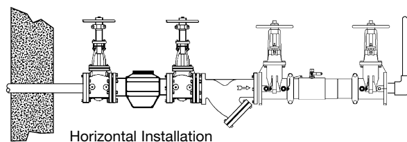
Horizontal Installation
