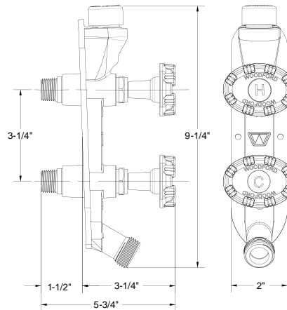
Model V122 Rough-In Dimensions
