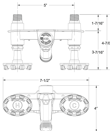
Model 122 Rough-In Dimensions
