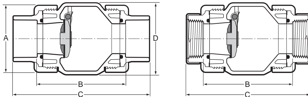
True Union Utility Spring Check Valve
