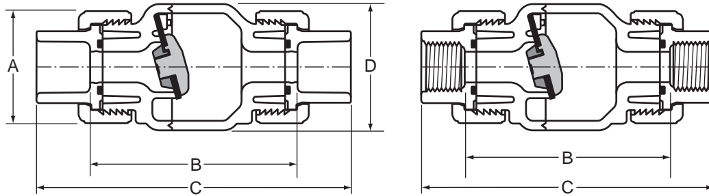
True Union Utility Swing Check Valve
