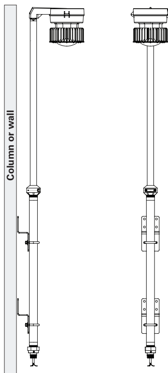
Column/wall mount
