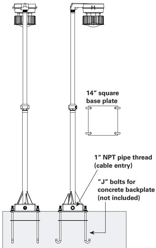
Base mount
