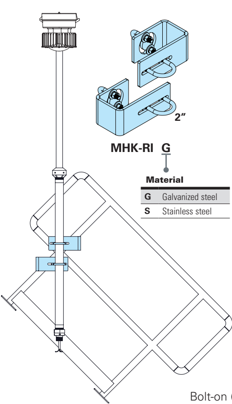
Universal rail mount – angular
