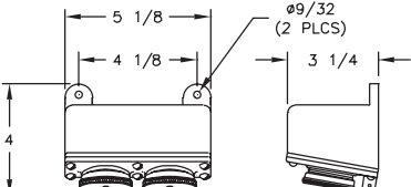
2592B/A-125
