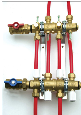
Manifold circuit sections rotate allowing tube to be routed from above or below the manifold offering the ultimate in job site flexibility.
